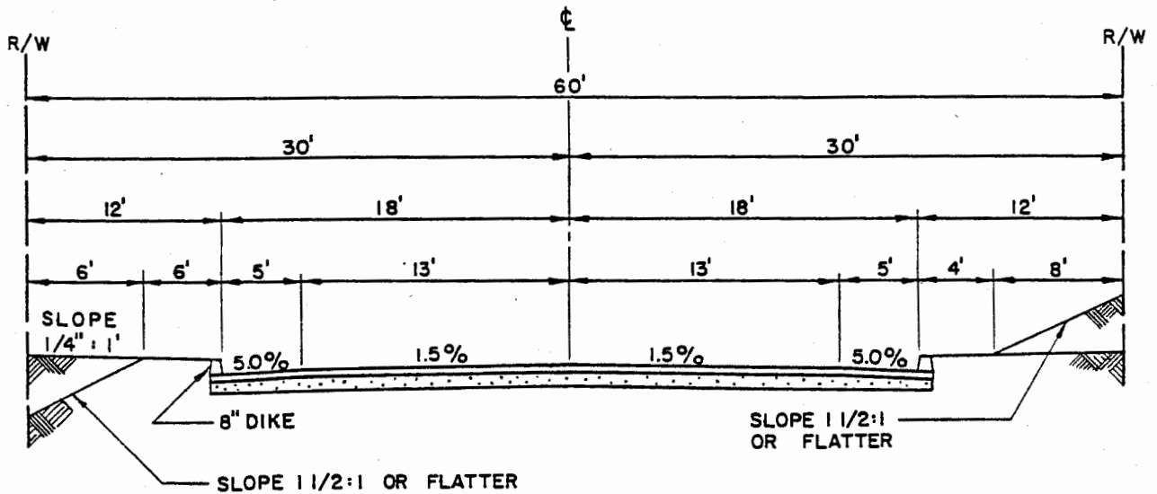
TYPICAL SECTION WHERE REQUIRED FOR DRAINAGE PURPOSES
