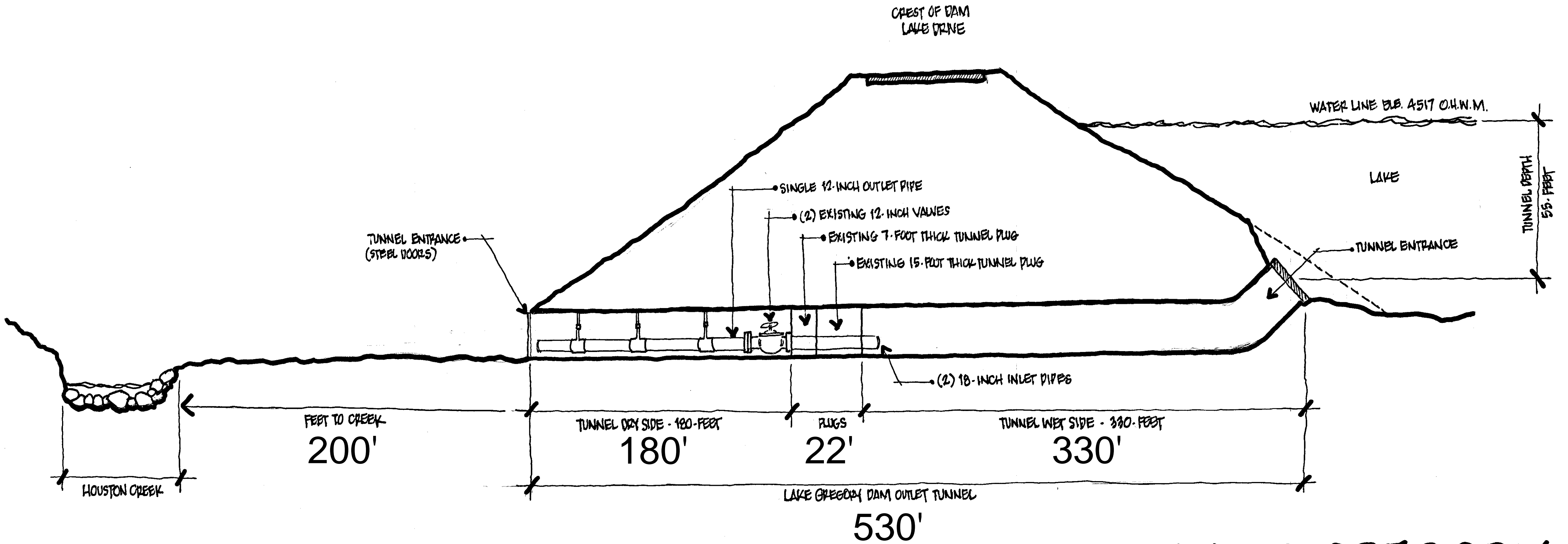
LAKE GREGORY. DAM OUTLET TUNNEL - EXISTING NOT-TO-SCALE
